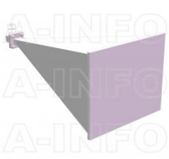
LB-75-25-C-7SP0 Standard Gain Horn Antenna 10-15GHz 25dB Gain 7mm
